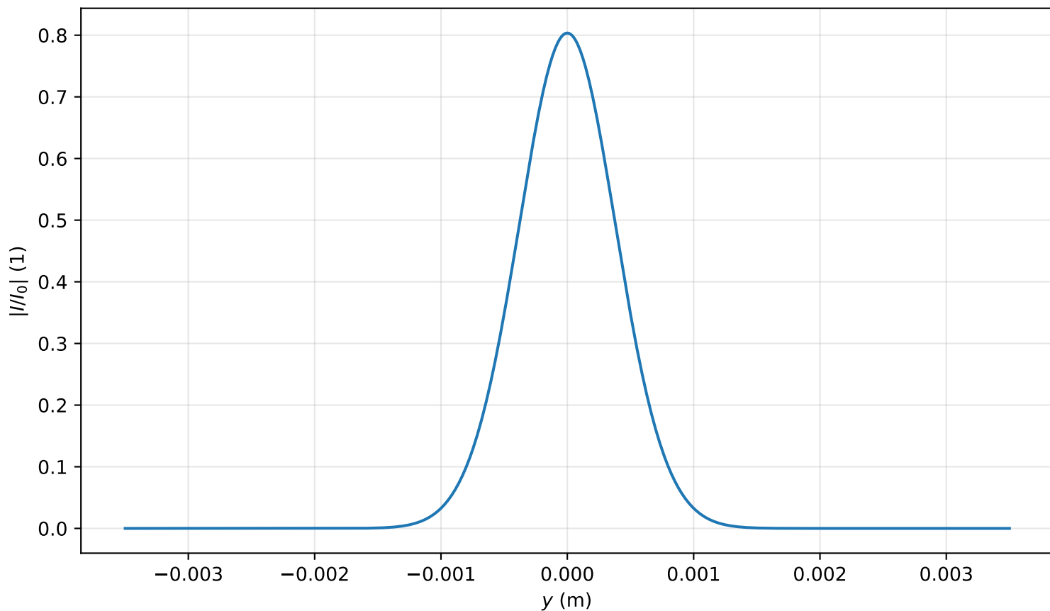
Intensity profile I(x=0, y, z=1.115)/I_0 , P_{in}=0.1P_{cr} , artificial time
